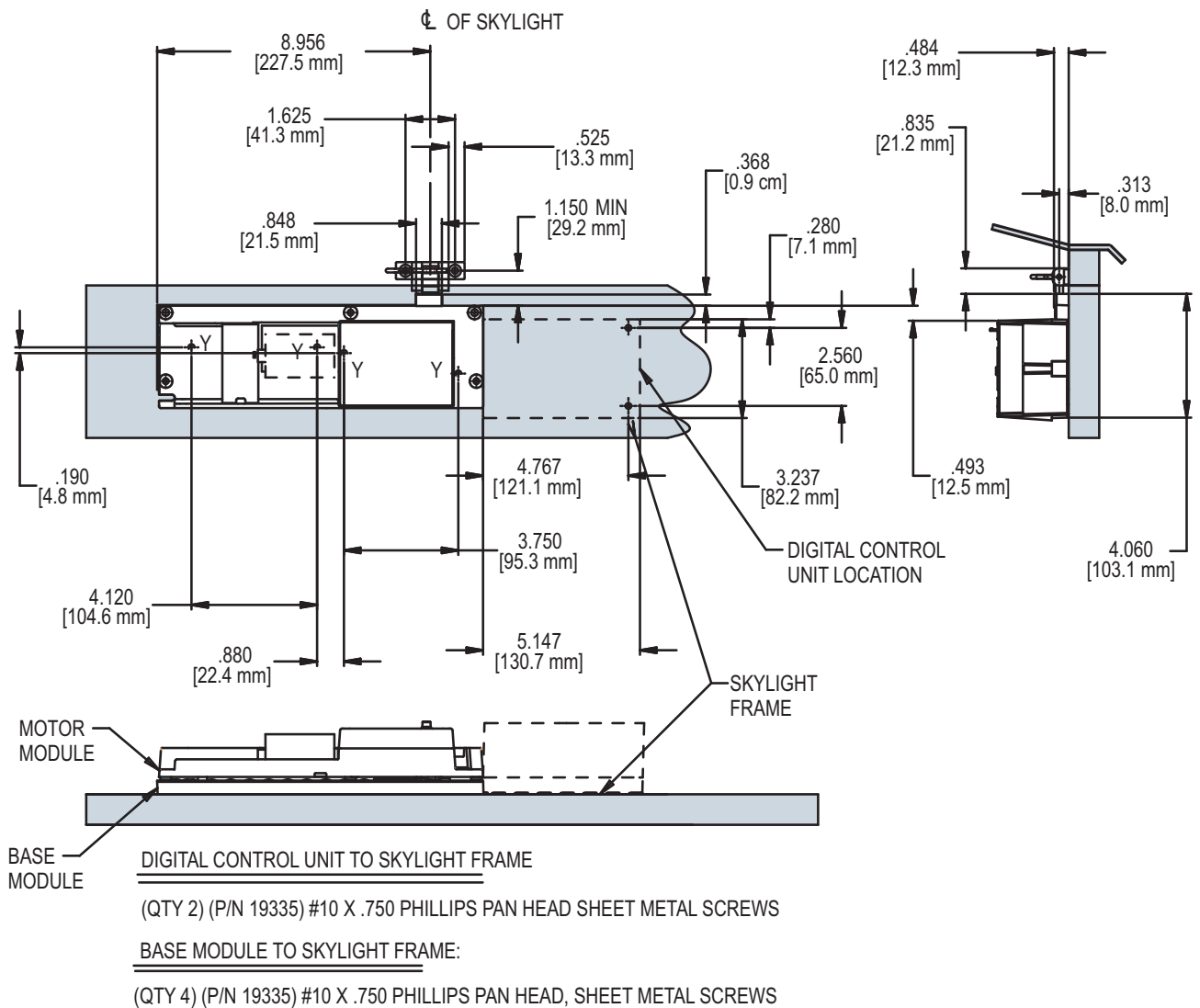
FIG. 2 SENTRY II HS MOUNTING ILLUSTRATION
