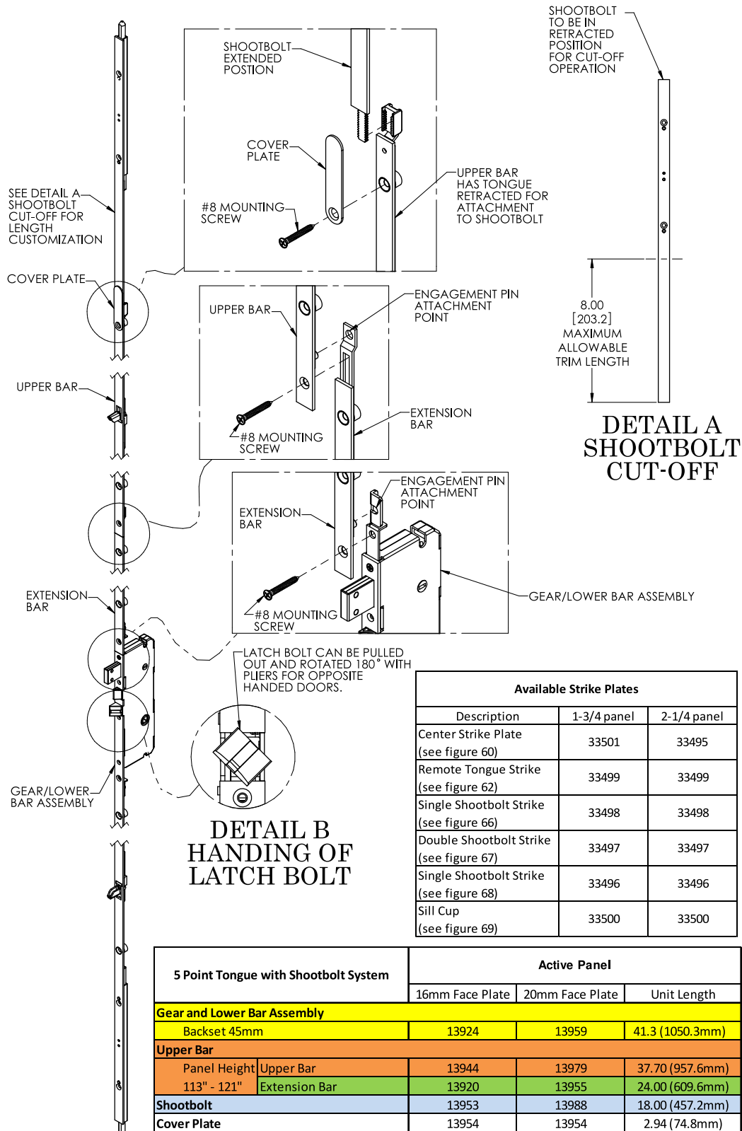
FIG. 26 SENTRY HINGED PATIO DOOR LOCKS 5 POINT TONGUE AND SHOOTBOLT ASSEMBLY FOR PANELS 113" TO 121"
