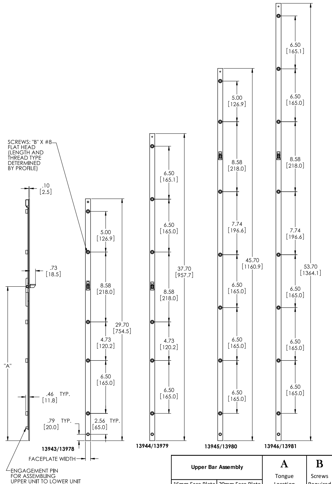
FIG. 30 SENTRY HINGED PATIO DOOR LOCKS 5 POINT TONGUE AND SHOOTBOLT UPPER BAR ASSEMBLY
