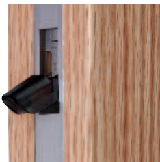
Tongue option fits standard 16 mm or 20 mm eurogrooves without additional remote lock processing
