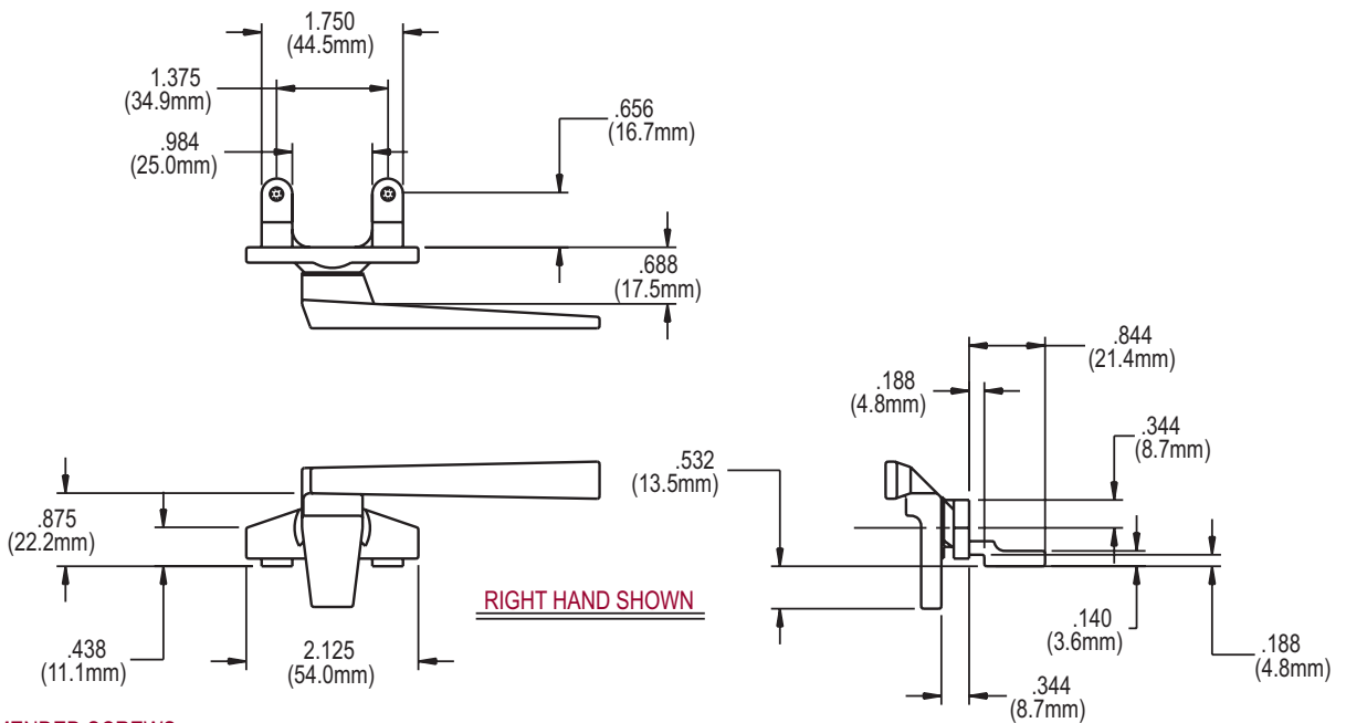
FIG. 5 25.76 CAM HANDLE (A-3 angle base)
