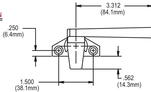
FIG. 2 25.29 CAM HANDLE (Offset Base)
