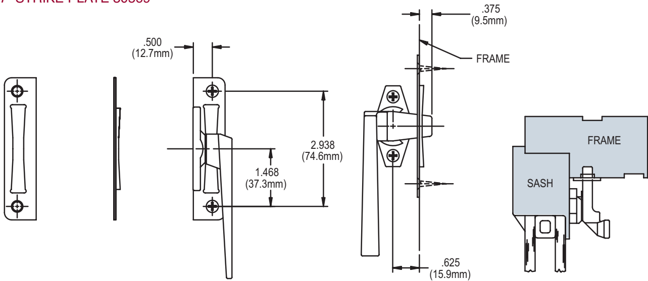
FIG. 7 STRIKE PLATE 30569
