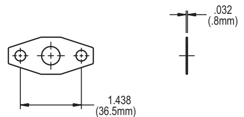
FIG. 11 GASKET 20408 (in-line base)
