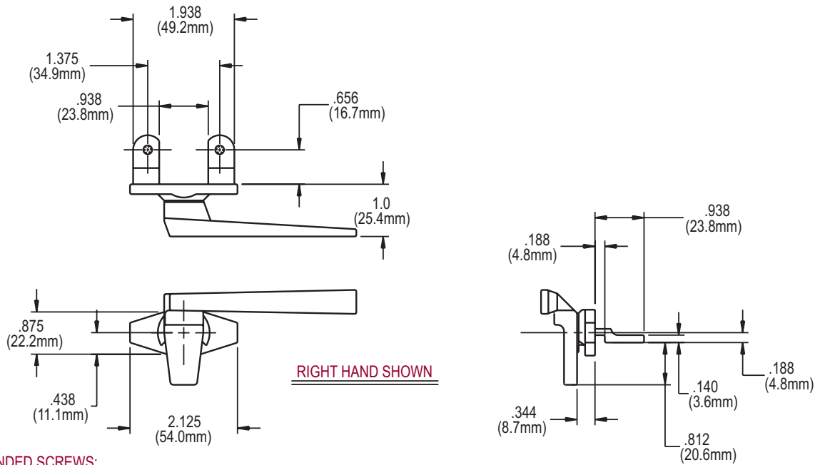
FIG. 4 25.39 CAM HANDLE (A-1 angle base)
