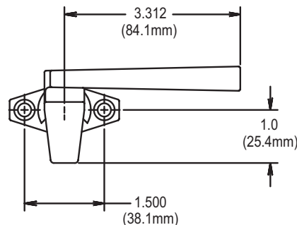
FIG. 3 25.31 CAM HANDLE (In-Line Base)
