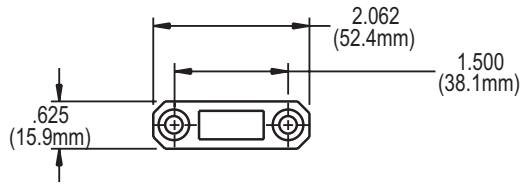
IN-LINE STRIKE HOUSING
