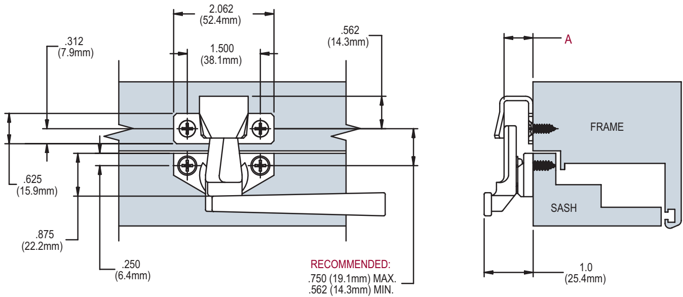
FIG. 6 25.80 CAM HANDLE FOR HOPPER WINDOWS 25.81 (Inline Base)
