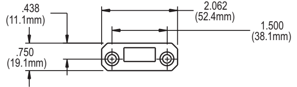
OFFSET STRIKE HOUSING
