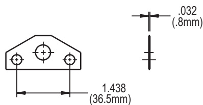
FIG. 10 GASKET 20556 (offset base)
