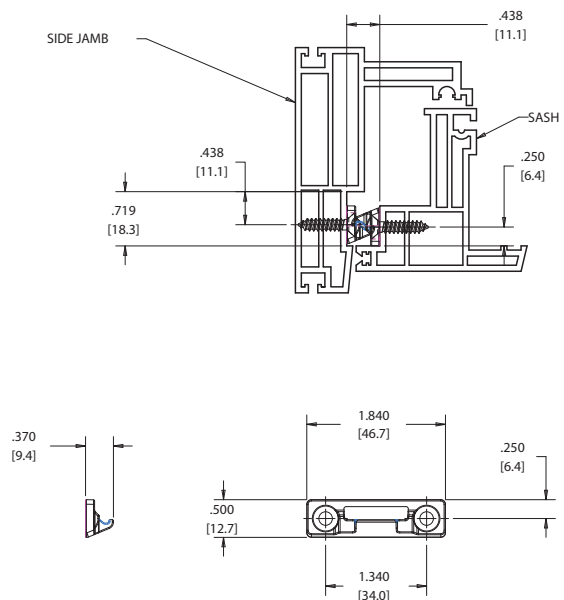
FIG. 3 22999.XX CONCEALED SNUBBER DIE CAST
