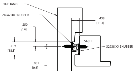
FIG. 2 32938.XX CONCEALED SNUBBER AND 21642.XX CONCEALED SNUBBER NEGATIVE AIR
