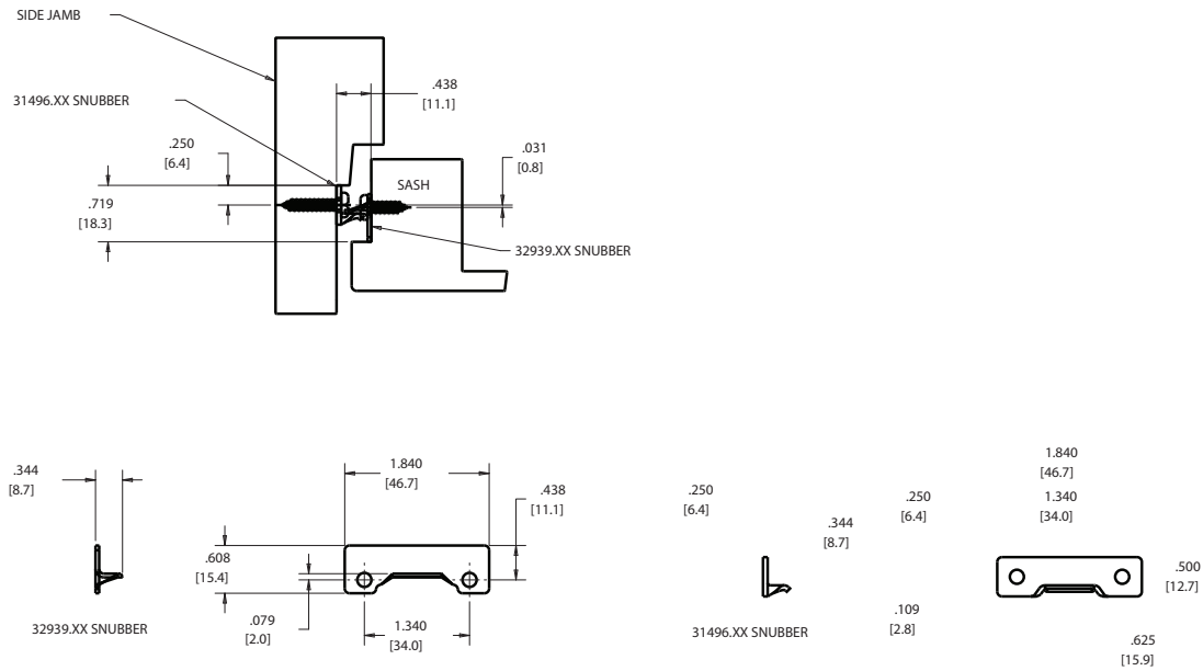
FIG. 1 32939.XX CONCEALED SNUBBER AND 31496.XX CONCEALED SNUBBER COMPRESSION
